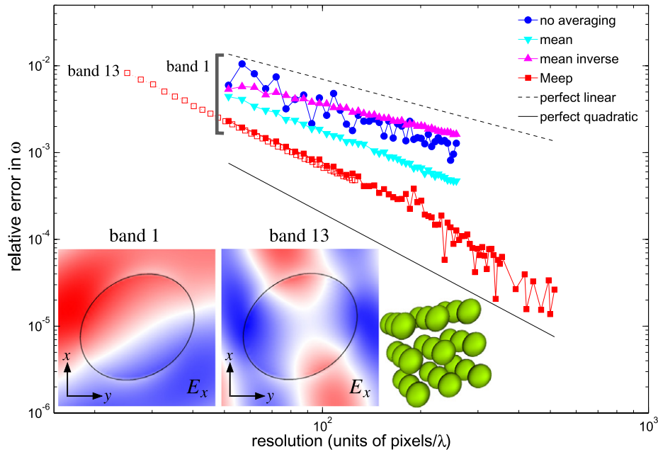
Fig. 6. Appropriate subpixel averaging can increase the accuracy of FDTD with discontinuous materials [33,34]. Here, relative error \Delta\omega/\omega (comparing to the “exact” \omega_0 from a plane-wave calculation [15]) for an eigenmode calculation (as in Section 5) for a cubic lattice (period a ) of 3d anisotropic- \epsilon ellipsoids (right inset) versus spatial resolution (units of pixels per vacuum wavelength \lambda ), for a variety of subpixel smoothing techniques. Straight lines for perfect linear (black dashed) and perfect quadratic (black solid) convergence are shown for reference. Most curves are for the first eigenvalue band (left inset shows E_x in xy cross-section of unit cell), with vacuum wavelength \lambda = 5.15a . Hollow squares show Meep’s method for band 13 (middle inset), with \lambda = 2.52a . Meep’s method for bands 1 and 13 is shown for resolutions up to 100 pixels/ a .
